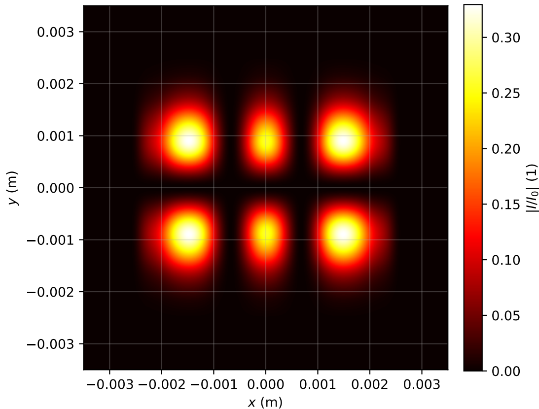
Intensity profile I(x, y, z = 3.184)/I_0 , P_{in}=1.0P_{cr} , artificial time
